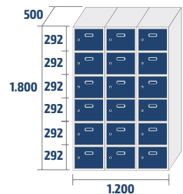
ECOB-40/3 PRO COD: 47104 74,3kg · 1,08m 3
